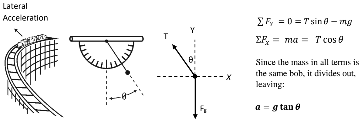
Figure 28 Pictorial and diagrammatic representations of using the sextant as a horizontal accelerometer.
