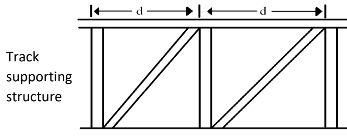
Figure 22 Detail of cross-members of a roller coaster structure.
